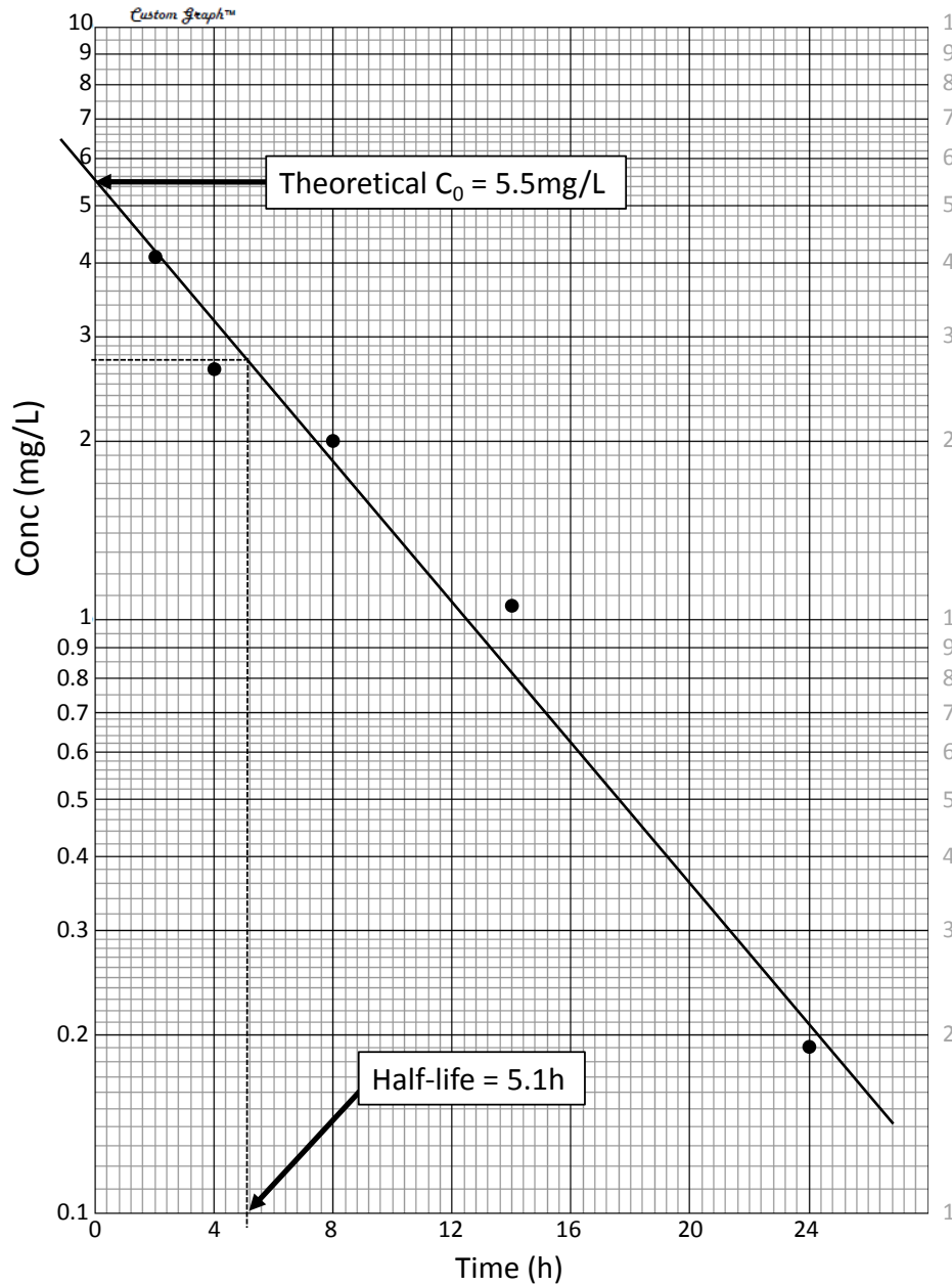
Figure 6.2 Concentration versus time on semi-log graph paper
