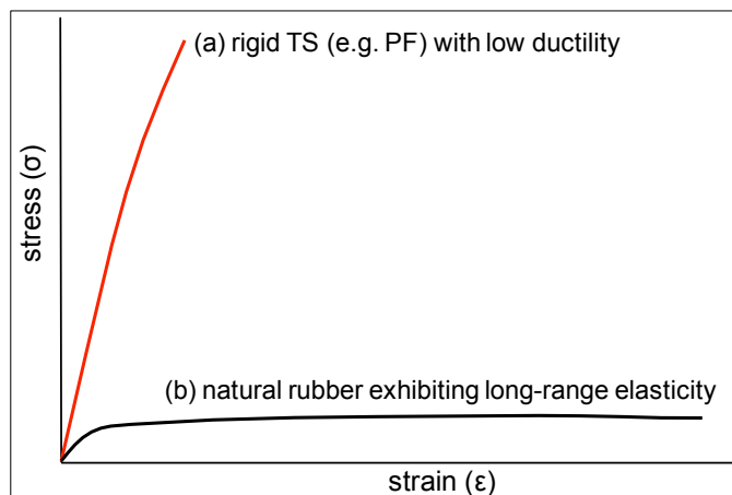
Figure 4.18 σ-ε curves for crosslinked polymers: (a) high X-link density, (b) low X-link density
