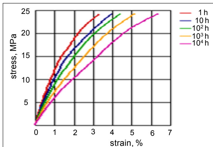
Figure 6.12 \sigma - \epsilon isochronous curves for Zytel 101L NC010 (PA66) (cond.) at 23 °C
