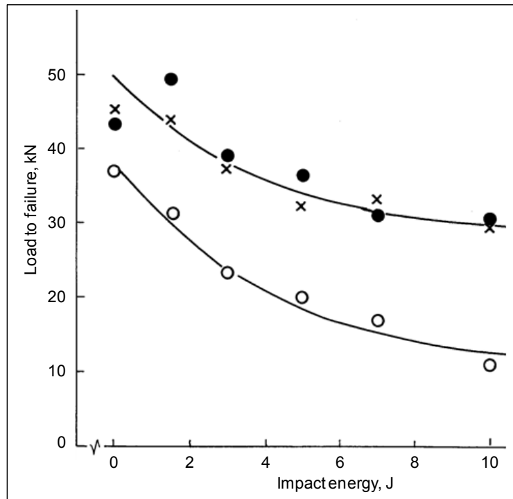
Figure 4.21 Compressive load to failure vs. incident impact energy for: (o) Panel A, (x) Panel B, and (•) Panel C CF/toughened epoxy (source: Akay & Hanna 1990)
