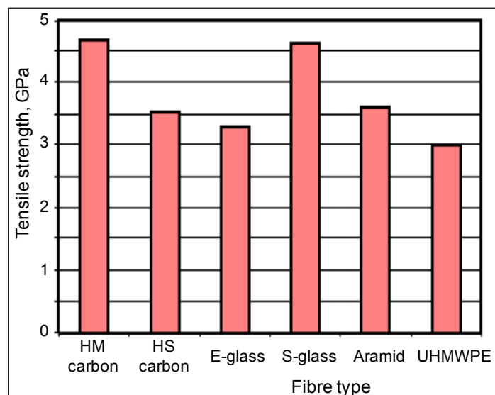
Figure 1.8 A comparison of tensile strength values for various fibres (source: Umeco, p. 6)
