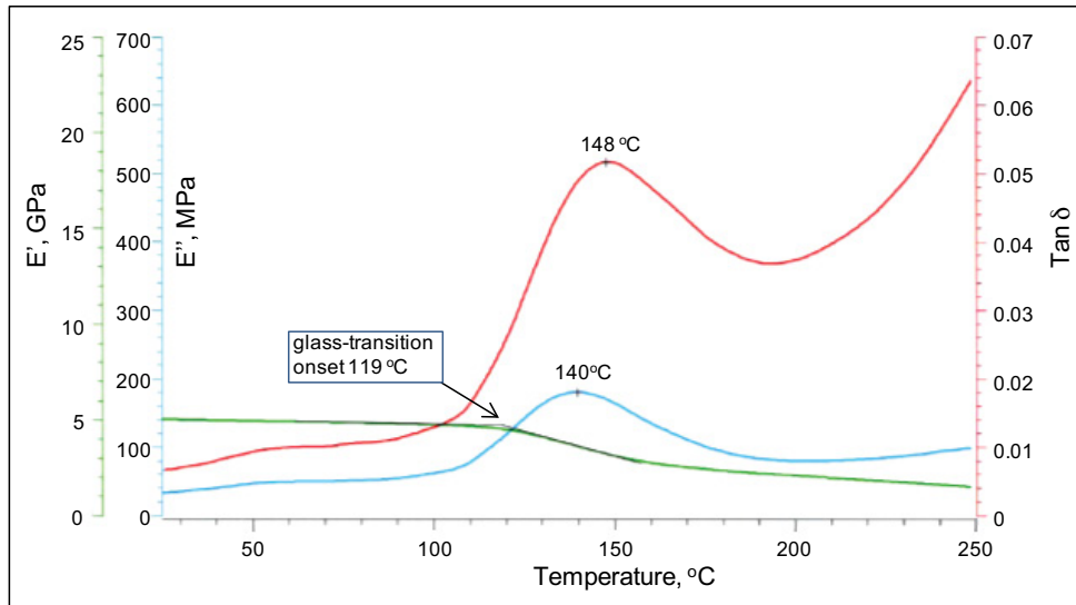
Figure 4.48 DMTA traces for PEEK/CF composite. The fibres are parallel to the specimen width (source: Netzsch GmbH)
