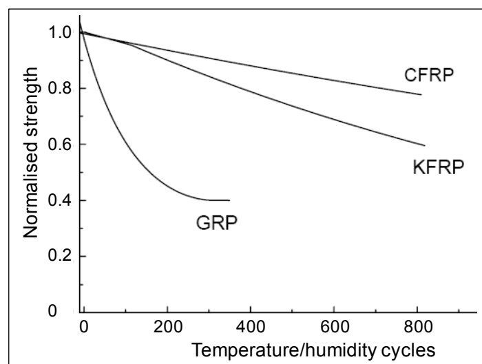
Figure 4.63 Reductions in the strengths of 0°/90° laminates of CFRP, GRP and KFRP as a consequence of temperature/humidity cycling. The cycle consisted of 12 hours at 2°C and 0 %RH, followed by 12 hours at 85°C and 100 %RH (source: Harris 1999, p. 163)
