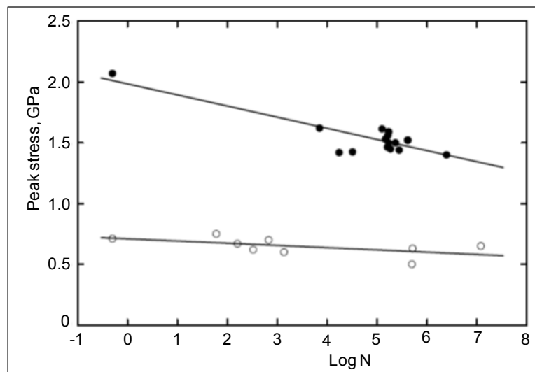
Figure 4.33 Stress/logN-life data for unidirectional composites of XAS/914 carbon/epoxy laminates reinforced with (●) continuous and (○) discontinuous fibres ( R = 0.1 ) (source: Harris et al. 1990)
